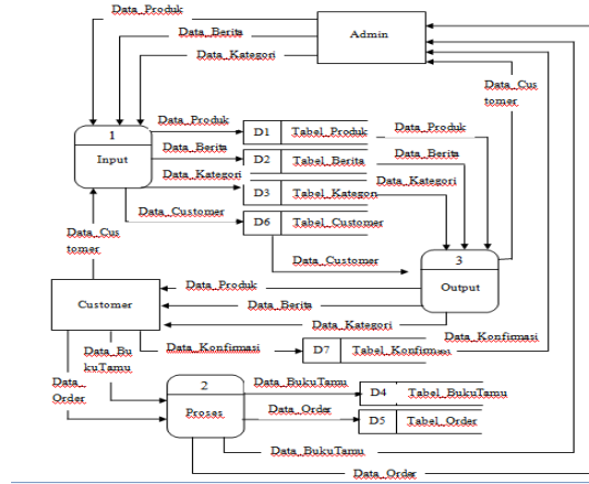
Gambar 3. DFD Level 0
