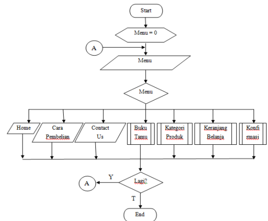
Gambar 5. Flowchart Program
