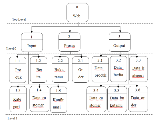
Gambar 2. Hierarchy chart
