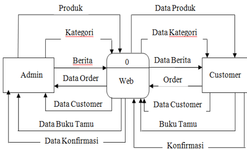
Gambar 1. ContextDiagram
